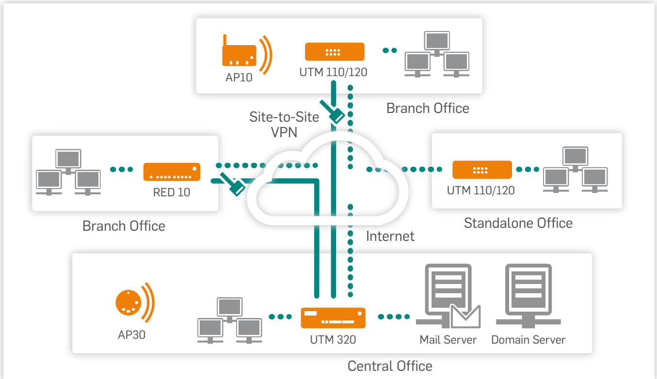
Deployment scenario of Sophos UTM 320
